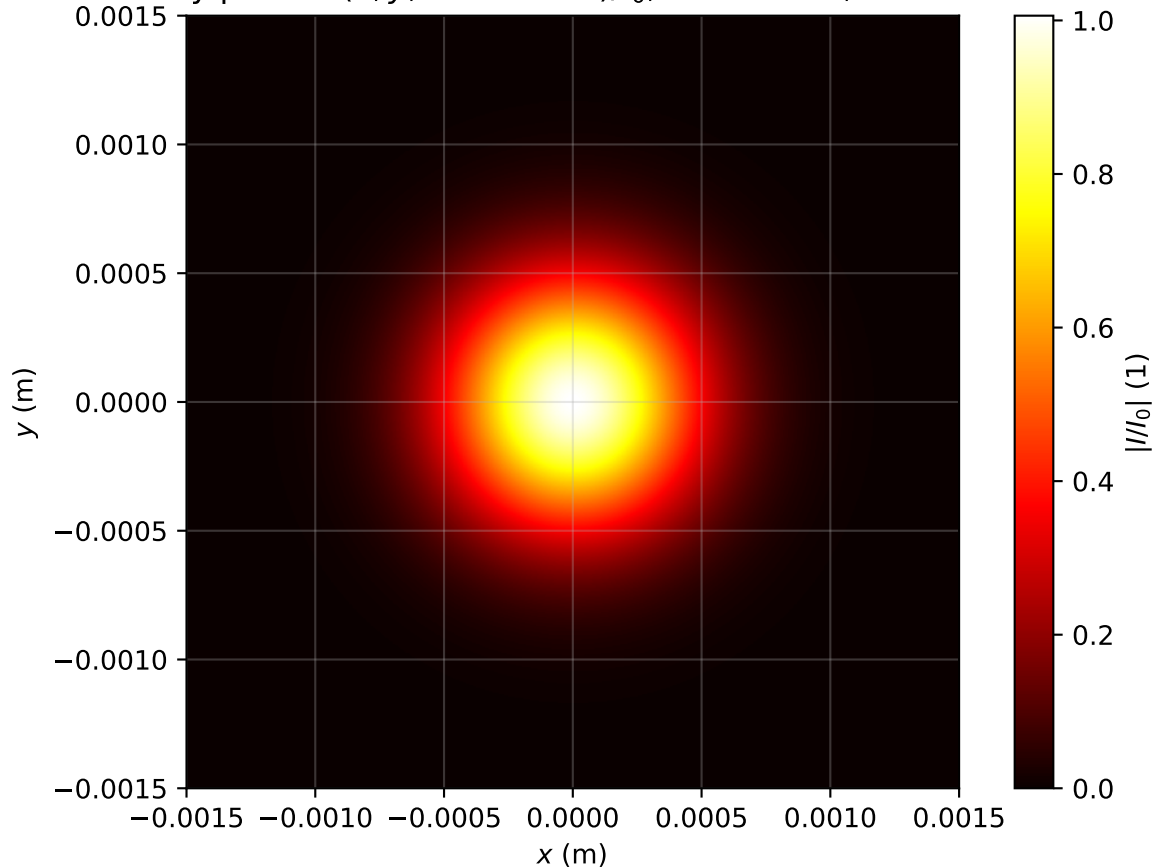
Intensity profile I(x, y, z = 0.159m)/I_0 , Pin=0.5Pcr, artificial time
